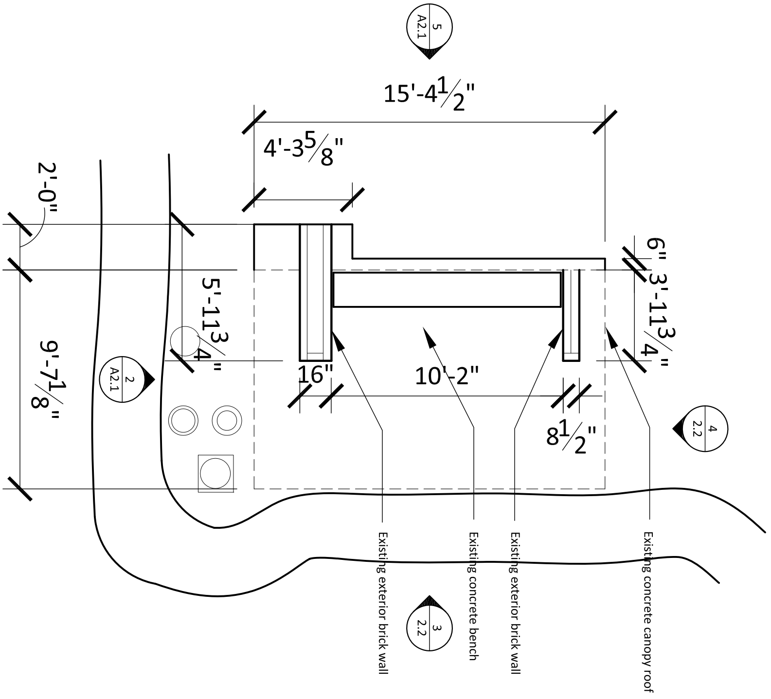
1 Plan of Existing Bus Stop Dimensions are approximate Scale: 1/4"=1'-0"
